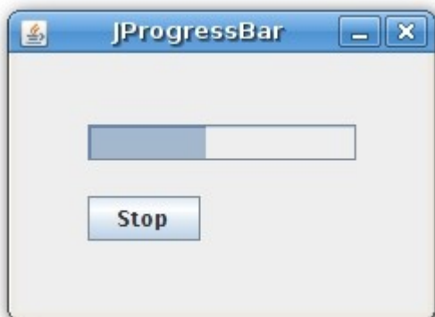
Figure: JProgressBar
